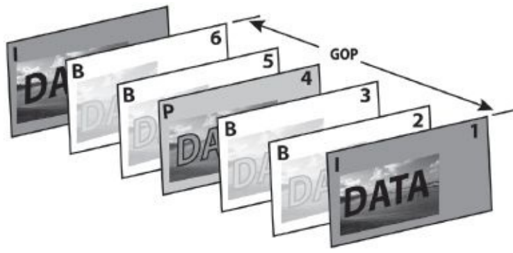
Fig. 5-33. Interframe compression means compressing several frames in a group (a group of pictures, or GOP). Only the I-frame is independently and completely stored; the P- and B-frames are calculated based on neighboring frames. The P-frame has about half as much data as the I-frame and the B-frames have one-quarter; compared to I-frames, they require more computing time to generate or view them. Pictured here is a 6-frame GOP used in the 720p version of HDV. The 1080i version uses a 15-frame “long GOP.” The longer the GOP, the greater the compression, and the more computing time and power that’s required to work with the material.
