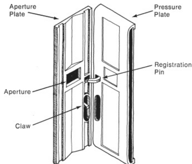
Fig. 6-3. Film gate with open pressure plate. Not all cameras use registration pins. (Carol Keller)
