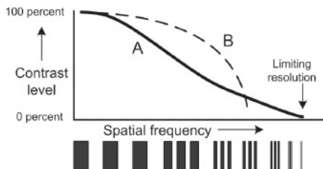
Fig. 5-28. An MTF (modulation transfer function) chart shows how well an imaging device (such as a lens) or a combined system (such as a lens plus a video camera, or a lens plus a film stock) can reproduce the contrast between black and white bars. On the left, the bars are far apart and the contrast is 100 percent. As we move to the right, the bars are thinner and more closely spaced; eventually they appear to blend together into gray (0 percent contrast). This point is the limiting resolution. System A
