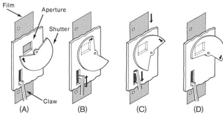
Fig. 1-32. The shutter and intermittent movement. (A) The claw holds the film in place during exposure. (B, C) The shutter rotates to block light from the film while the claw moves up to pull down the next frame. (D) The claw freezes in position to hold the next frame steady for exposure. (Carol Keller)
