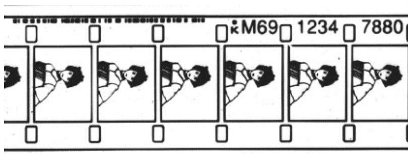
Fig. 7-9. 16mm key numbers and Keycode. (Eastman Kodak Company)
