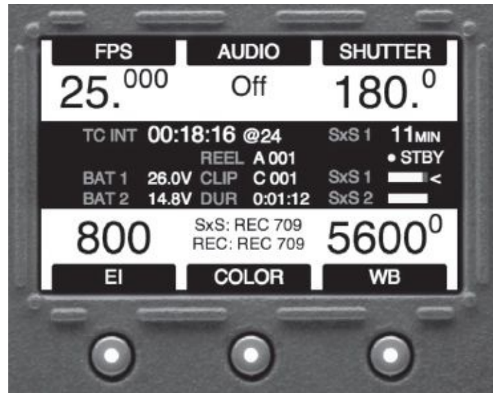
Fig. 3-17. This panel on the ARRI Alexa displays key camera settings. Starting in the lower right and moving clockwise, you can see the white balance is set to 5600 degrees kelvin; the EI (same as ISO) is set to 800; the frame rate is set to 25 fps; and the shutter angle is set to 180 degrees. Shutter angle is simply another way of expressing the shutter speed; a 180-degree shutter is open for half of each frame, so the shutter speed at 25 fps is \frac{1}{50} second. (ARRI, Inc.)
