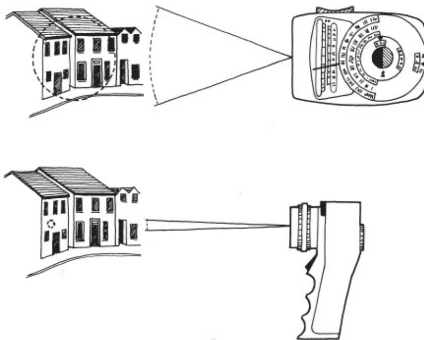
Fig. 7-15. (top) A typical reflected light meter has a wide angle of acceptance (about 40 degrees here) and averages areas of differing brightness. (bottom) A spot meter (pictured here with a 5-degree angle of acceptance) can isolate a small area in the subject. (Carol Keller)
