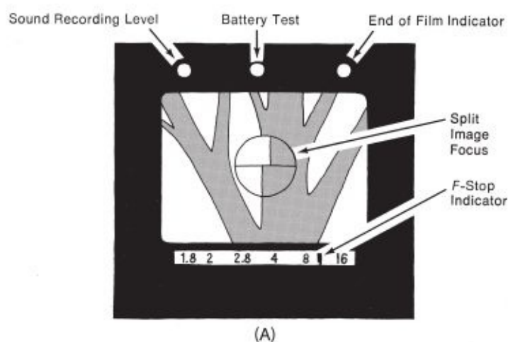
Fig. 6-6. Ground glass viewfinder screen typical of 16mm cameras. Note the safe viewing area, which provides warning of things just outside the frame. Horizontal marks near the edge of the frame indicate top and bottom frame lines when shooting for 1.85:1 widescreen aspect ratio. On some 35mm cameras, the viewfinder includes a magnification system to enlarge the frame for critical focusing, and a lens to unsqueeze an anamorphic image. (Carol Keller)
