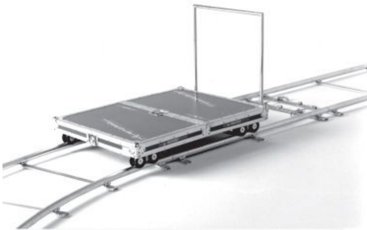
Fig. 9-44. Briefcase dolly. Can be used with straight or curved track or on bare floor. The dolly platform folds up, becoming a thin carrying case for travel. (Fletcher Chicago/Egripment USA)
