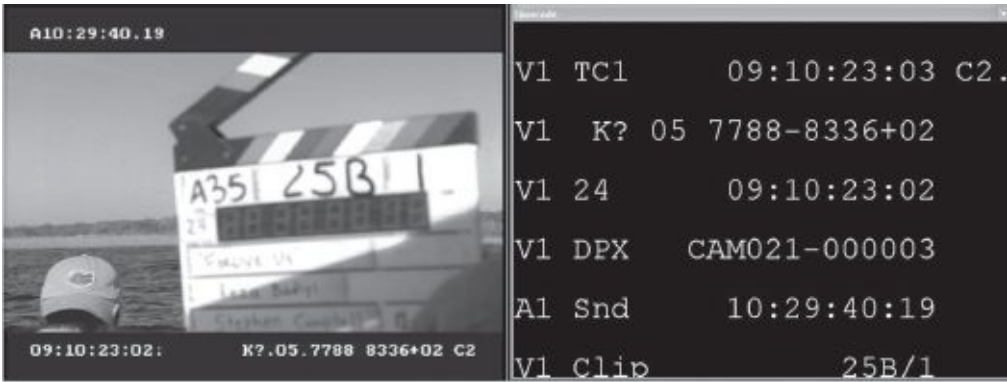
Fig. 16-9. Telecine and video data. This Avid display shows the data that the NLE is tracking, which includes: the timecode of the video transfer (09:10:23:03), the pulldown phase (C2), the film keycode
