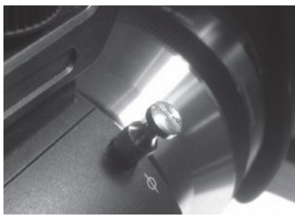
Fig. 4-14. Some cameras have a hook to attach a tape measure when doing tape focus. The \Phi indicates the position of the sensor (or the film plane in a film camera). (Steven Ascher)
