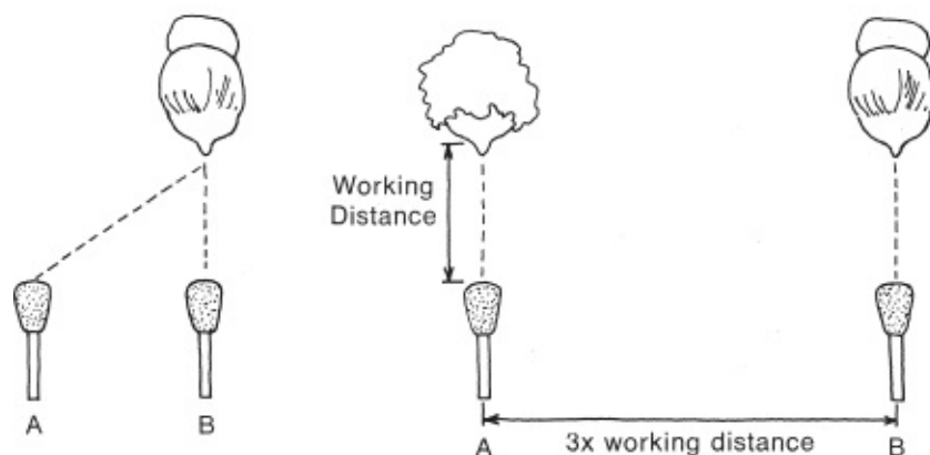
Fig. 11-13. Multiple microphones. (left) Distance from the woman to microphone A is only slightly longer than distance to microphone B, leading to possible phase cancellation. (right) Separation between microphones is three times the distance from each mic to its sound source. Now the distance between microphone A and the woman at right is sufficient to minimize the chance of phase cancellation. (Carol Keller)
