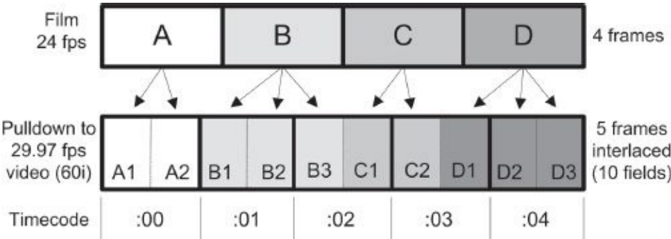
Fig. 16-10. This shows the relationship of pulldown and timecode in an A-frame film transfer using normal pulldown. See also Fig. 14-31.
