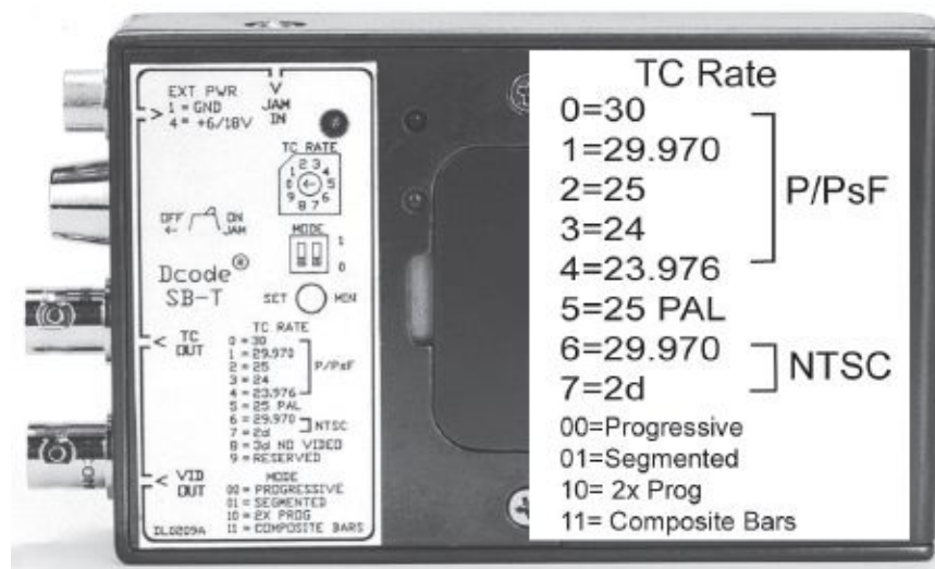
Fig. 11-20. Timecode generator. The Denecke SB-T reads, generates, and jams to all standard frame rates. Outputs timecode and video sync in PAL and NTSC, as well as trilevel sync for HD. Enlargement shows available frame rates. (Denecke, Inc.)
