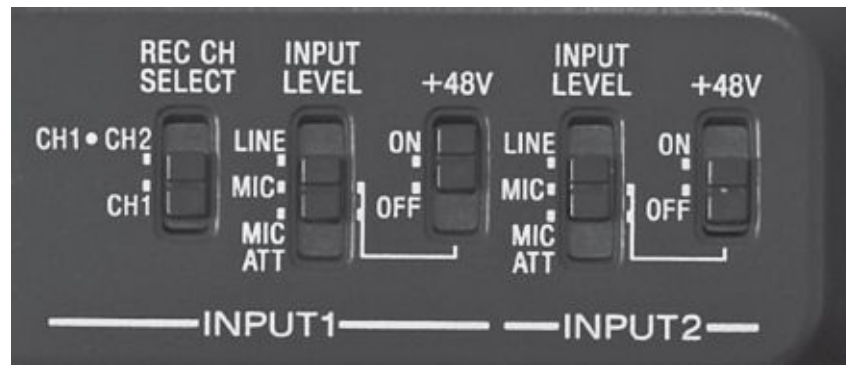
Fig. 10-31. Audio input selector on a Sony camcorder. Note choice of input level including Line, Mic, and Mic ATT (short for “attenuator,” this reduces the level by 20 dB for loud situations). When mic input is selected, you can choose “+48 volt” for condenser mics that require phantom power or select Off for self-powered condensers and dynamic mics. (Sony Electronics, Inc.)
