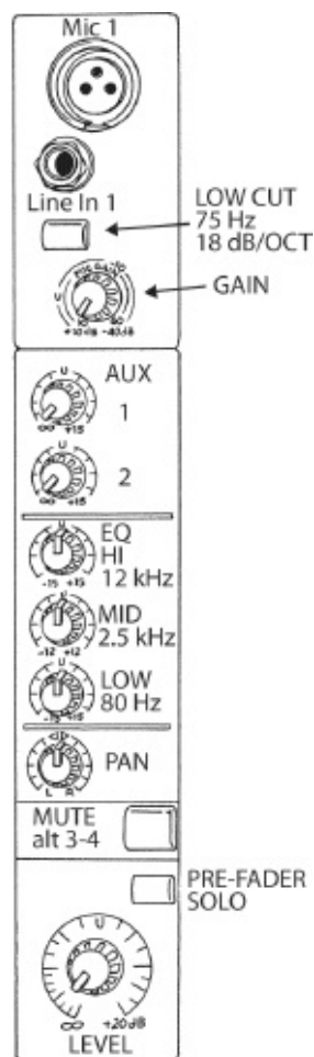
Fig. 15-5. Channel strip from Mackie 1202-VLZ3 mixer. See text. (Robert Brun)
