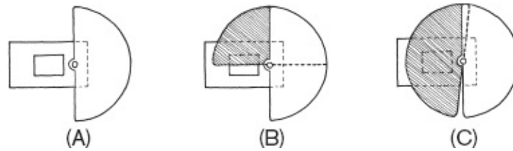
Fig. 6-4. Variable shutter. (A) A 180-degree shutter shown fully open. The small rectangle represents the aperture. (B) To close the shutter, an adjustable disc (shaded) swings out; shown here, it forms a 90-degree opening. (C) The shutter is almost completely closed. (Carol Keller)
