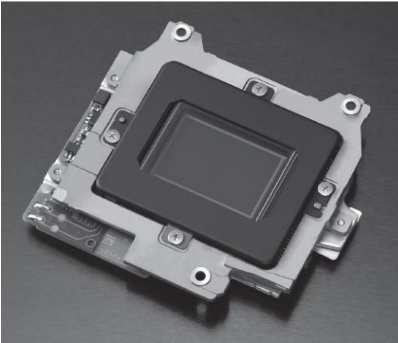
Fig. 2-6. DSLR sensor from a Nikon D5100. The sensor size is Nikon DX, which is one of the APS-C formats. (Nikon, Inc.)
