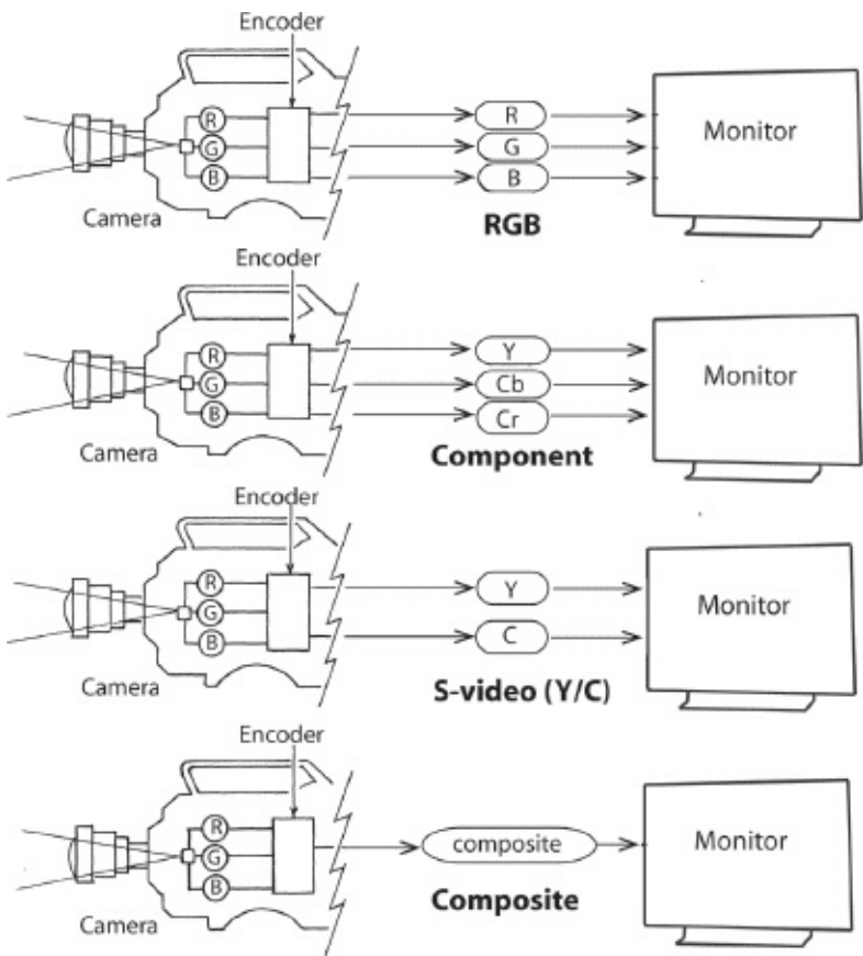
Fig. 5-14. RGB, component, S-video, and composite video systems vary in the paths they use to convey the video signal from one piece of equipment to another. For systems that use multiple paths, the signal is sometimes sent on multiple cables, but often the various paths are part of one cable. See text. (Robert Brun)
