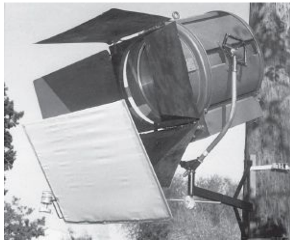
Fig. 12-27. A silk being used to cut the bottom half of the light beam; this evens out the illumination close to and far from the light. This light is attached to the telephone pole using a poultry bracket. (Matthews Studio Equipment, Inc.)
