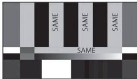
Fig. C. With SMPTE HD bars, when setting chroma (also called saturation or "color") with a monitor in blue-only mode, these four bars should have the same brightness.
