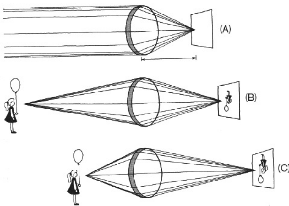
Fig. 4-1. Focal length. (A) The rays from a point source of light at infinity are parallel when they strike the lens. The distance from the lens to the focal plane (where the rays are brought back to a point) is the focal length . (B) The photographic lens forms an upside-down image flipped from left to right. (C) The closer an object is to the lens, the farther from the lens the rays converge and the larger the object appears on the film. (Carol Keller)
