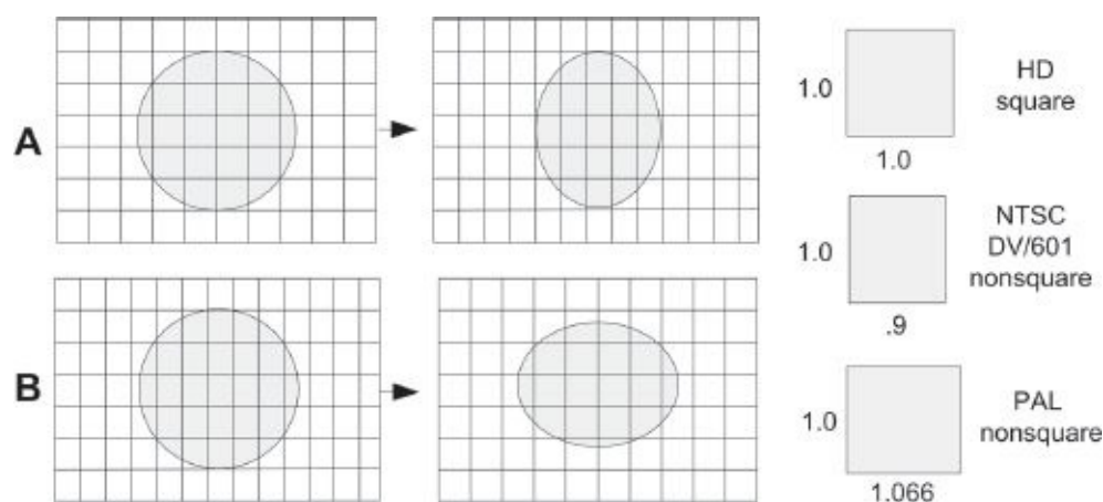
Fig. 5-27. Pixel aspect ratio. When converting between formats or systems that have different-shaped pixels, the image can become distorted if adjustments aren't made. (A) An image created in a square pixel format (such as HD or any computer graphics application) can look horizontally squeezed when imported into standard definition NTSC-based formats, which use tall, nonsquare pixels. (B) An image created in an NTSC-based format can look horizontally stretched when shown on a computer monitor (which displays square pixels) or imported into a computer graphics application. Note that settings vary, and some apps compensate automatically, so your results may not be distorted or may be distorted in different ways. The NTSC and PAL pixel aspect ratios indicated on the right are for nonwidescreen formats.
