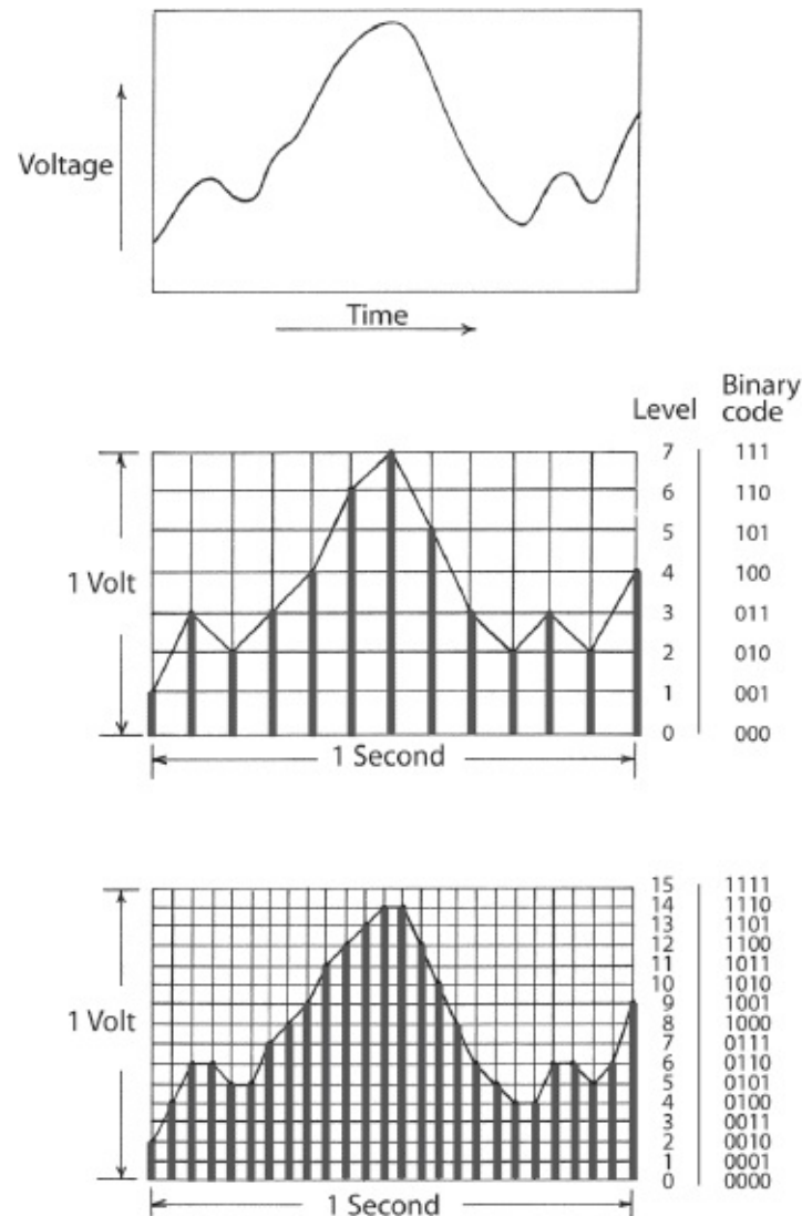
Fig. 10-3. Digital recording. (top) The original analog signal. Note that the voltage level changes continuously over time. (middle) To record the signal digitally, we take samples (measurements) at regular time intervals (the vertical lines). The level of the signal at each sample is measured according to a level scale (the horizontal lines). The total number of units in the scale is determined by the number of bits in the system; a three-bit system is pictured here. Samples can only be measured in one-unit increments . A measurement that falls between, say, level 2 and level 3 must be rounded down to 2 or up to 3. (bottom) This has twice as many samples in the same period of time (higher sample rate ). And by using more bits (four instead of three), we can measure each sample with greater precision . This is a higher-resolution recording that better approximates the shape of the original analog signal. (Robert Brun)
