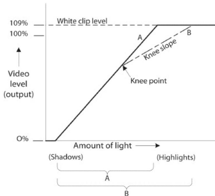
Fig. 5-1. The video sensor’s response to light. The horizontal axis represents increasing exposure (light) from the scene. The vertical axis is the level of the resulting video signal that the camera produces. Line A shows that as the light increases, so does the video level—until the white clip is reached, at which point increases in light produce no further increase in video level (the line becomes horizontal). With some cameras, a knee point can be introduced that creates a less steep knee slope to the right of that point (Line B). Note how this extends the camera’s ability to capture bright highlights compared to A. This graph is deliberately simplified. (Steven Ascher)
