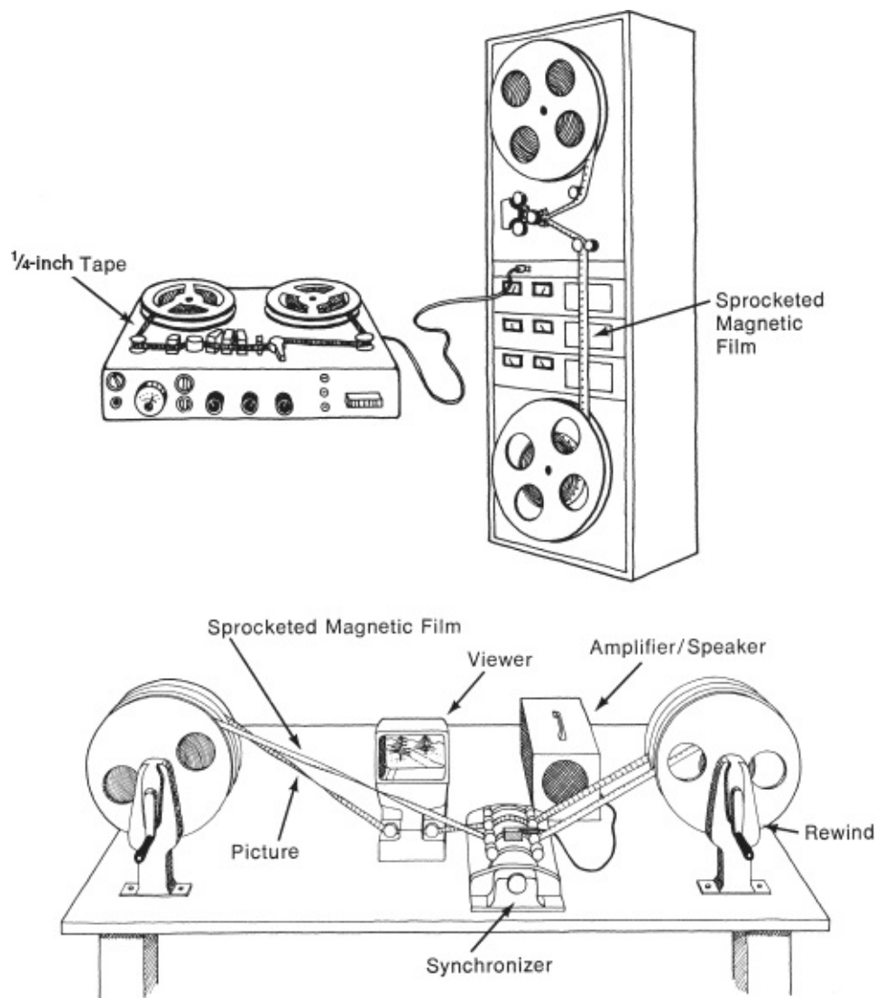
Fig. 1-42. Traditional film editing. (top) Sound recorded in the field (represented here with a 1/4-inch tape deck) is transferred to sprocketed magnetic film for editing. (bottom) The mag film can then be edited with the picture in frame-for-frame correspondence. Most of the equipment shown here is now rarely used. (Carol Keller)
