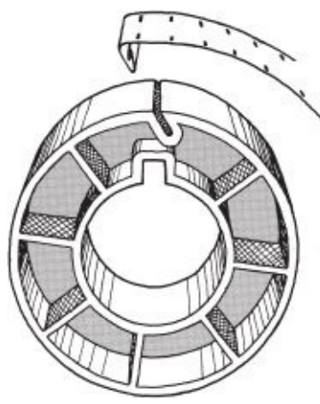
Fig. 6-12. Attaching the film to take-up core. Fold the film over itself and insert it in the slot. Position the slot as illustrated—angled against the direction of the take-up to keep the film from slipping out. Rotate the core to wind up several turns of film. Some magazines take up with emulsion facing in and others face out. (Carol Keller)
