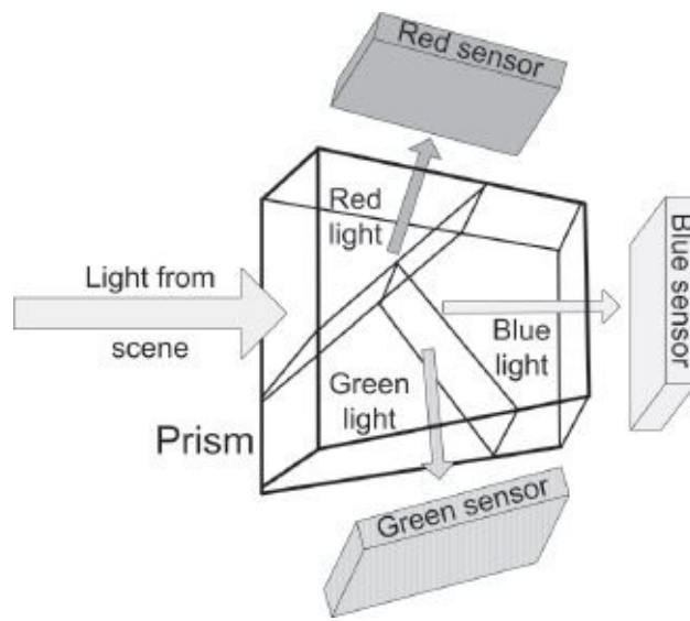
Fig. 1-14. In a three-chip camera, light entering through the lens strikes a prism that divides it into its red, green, and blue components. Each is captured by a separate sensor. (Steven Ascher)
