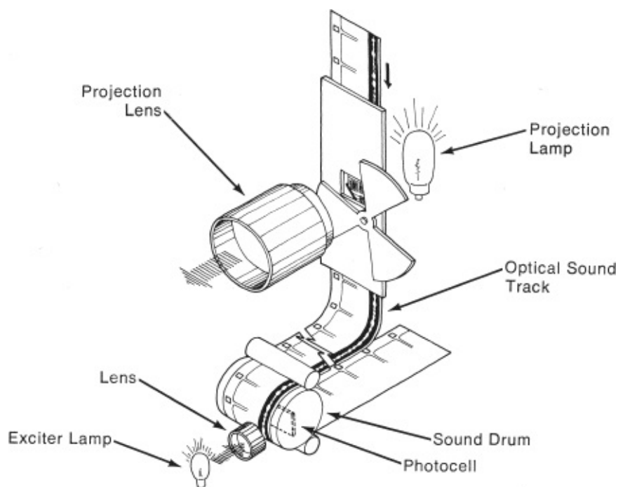
Fig. 16-15. Film projector and optical sound. Light from the exciter lamp shines through the optical sound track. The resulting variations in the light are registered by the photocell (shown in cutaway). In 16mm, the optical sound reader is separated from the film gate where the image is projected by 26 frames. (Carol Keller)
