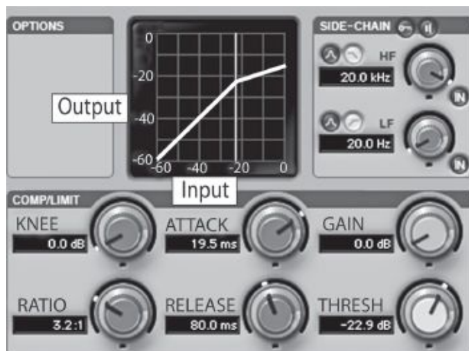
Fig. 15-15. Compressor/limiter. This DigiRack plug-in has a graph that shows the relationship of the sound level going into the compressor (the horizontal axis) and the sound level coming out of the compressor (the vertical axis). With no compression, output equals input. In this figure, audio levels above the -22 dB threshold will be compressed (reduced in volume). It's interesting to compare this to Fig. 5.1 , which shows a graph with a similar slope used to compress video levels. (Avid Technology, Inc.)
