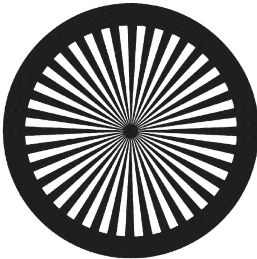
Fig. 4-28. Focus chart. Get a full-sized chart or use this one in a pinch. (Schneider Optics)
