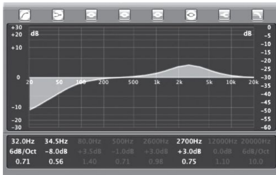
Fig. 15-17. An equalizer can boost different frequency bands (above the 0 dB line) or diminish them (below the line). The controls at the bottom of this Apple Logic equalizer allow you to select the center of each frequency band, how wide the band is, and how much to raise or lower the sound level. The EQ shown here is a basic one for improving the clarity of speech tracks by boosting the midrange and rolling off the bass (compare it with Fig. 10-21B ). Equalization should always be done by ear and not by formula. (Apple, Inc.)
