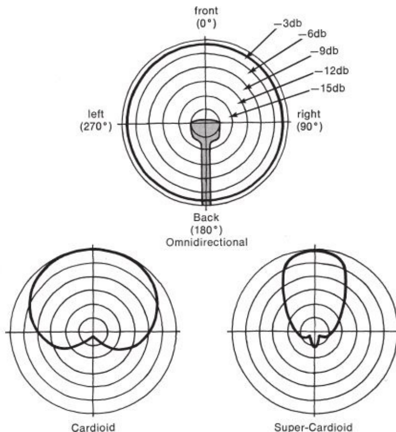
Fig. 10-20. Polar diagrams indicating the sensitivity of omnidirectional, cardioid, and supercardioid
