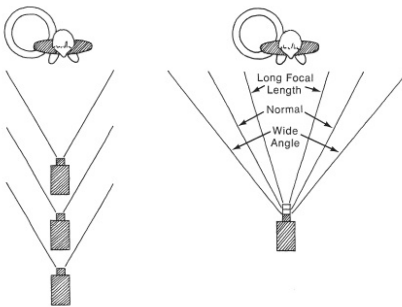
Fig. 4-2. Angle of view and focal length. (left) Keeping the angle of view constant, moving closer to the man (dollying in), makes him appear larger. (right) Keeping the camera in the same position while using increasingly longer focal lengths also makes the man larger but decreases the angle of view. See the results in Fig. 4-3 . (Carol Keller)
