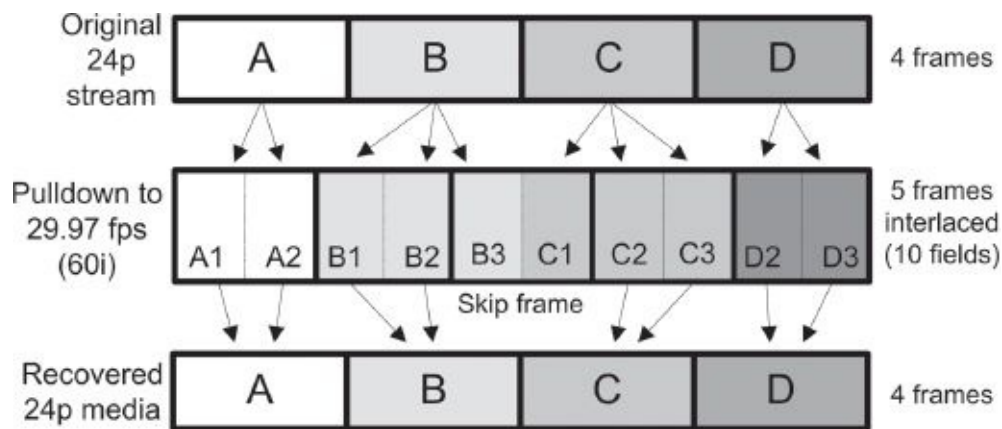
Fig. 14-32. Advanced (2:3:3:2) pulldown. Note the difference between this and Fig. 14-31 . Instead of deleting separate fields B3 and D1 to re-create the 24p media, here we delete the entire third frame (B3 and C1), which makes for a cleaner, simpler reverse pulldown process.
