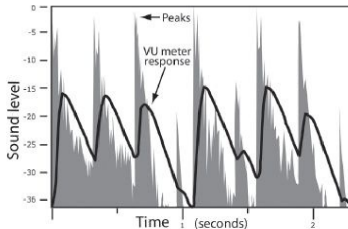
Fig. 11-9. Peak level and the VU meter. The gray area represents the sound level of a drumbeat, with its short, percussive peaks. The black line is the response of a VU meter. Note that the VU meter lags behind the actual spikes in level, and it doesn't rise as high or drop as low as the quick peaks and valleys. The VU meter indicates an average level that gives a good sense of how loud something sounds but is often significantly lower than the actual peaks. (From http://en.wikipedia.org/wiki/VU_Meter )
