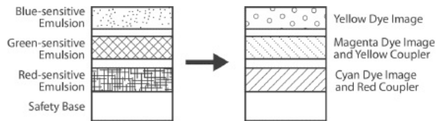
Fig. 7-4. Color negative before (left) and after processing. Yellow and red couplers are found in the green- and red-sensitive emulsions to compensate for deficiencies in color absorption of the magenta and cyan dyes.
