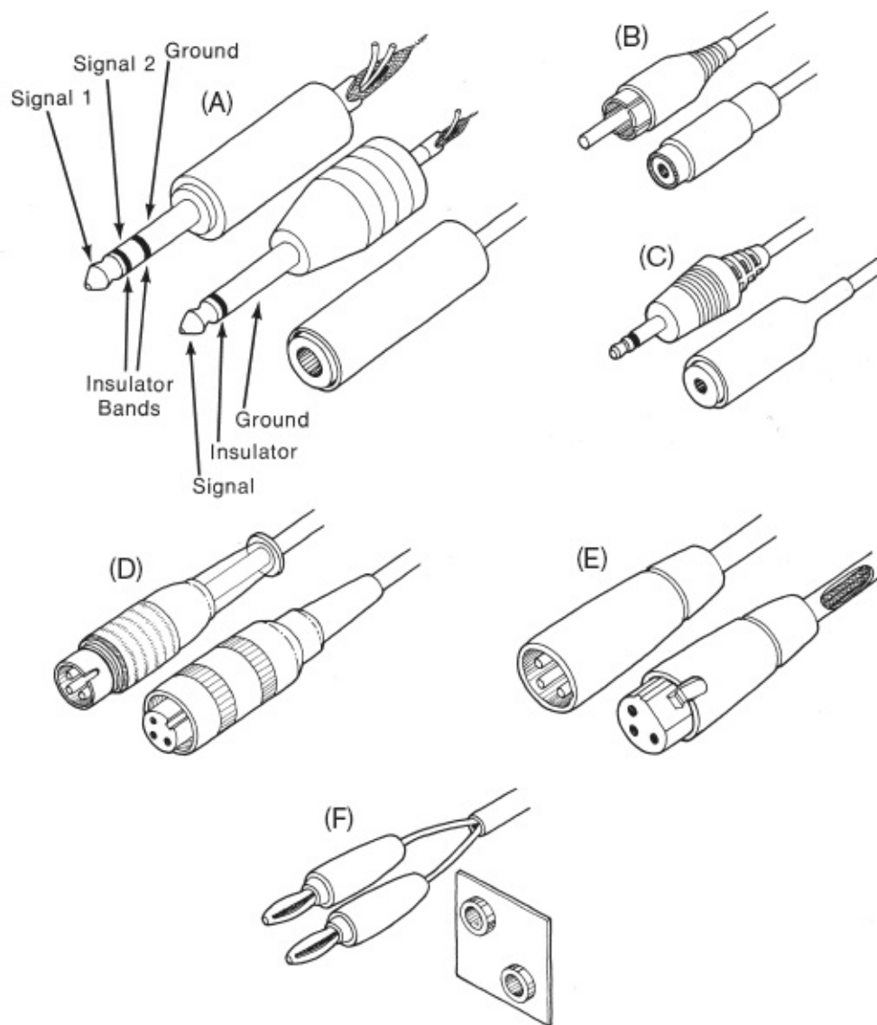
Fig. 10-32. Audio connectors. (A) \frac{1}{4} -inch males and female. A three-contact (also called TRS) stereo plug is at left, a two-contact (TS) mono plug is in the center. The three-contact version can be used for balanced cables. (B) RCA or phono male and female. (C) Mini phone or simply mini male and female. This is a miniaturized version of the \frac{1}{4} -inch connector (diameter is \frac{1}{8} inch—3.5mm—instead of \frac{1}{4} inch). There is a stereo version of this plug, recognizable by the two black insulator bands (see A). There is also a sub-mini plug that's even smaller—2.5mm. (D) Three-pin Tuchel male and female. The sleeve on the female engages the threads on the male. This Tuchel is a variant of a DIN connector. (E) Three-pin XLR or Cannon connectors. The male and female snap together. Both XLR and Tuchel connectors may have more than three pins. The female XLR is pictured with the insulation cut away to show the balanced or stereo cable with the two signal wires encased in the sheathlike ground. (F) Banana plugs and jacks. For more audio and video connectors, see Figs. 3-14 , 5-14 , and 10-13 . (Carol Keller)
