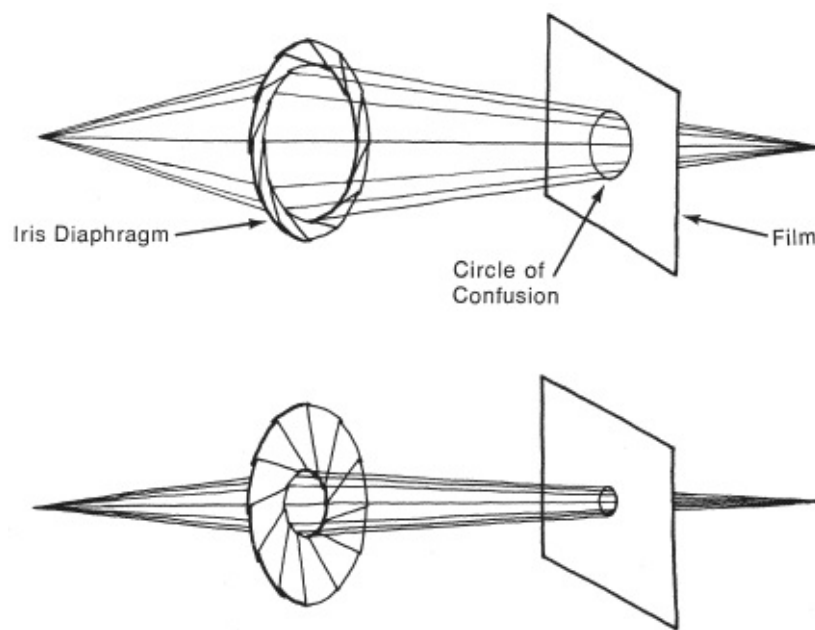
Fig. 4-12. Stopping down the lens increases depth of field. (top) Circle of confusion at wide aperture. (bottom) As the iris diaphragm closes, the diameter of the cone of light gets smaller and so the circle of confusion is smaller. (Carol Keller)
