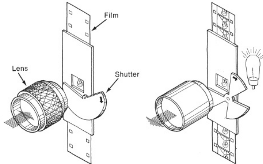
Fig. 1-31. The camera and the projector. The camera (left) draws in light to capture an image of the world on film; the projector (right) throws the image back onto a screen. (Carol Keller)
