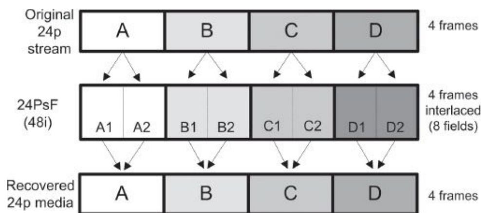
Fig. 14-30. Progressive segmented frame (PsF). The top line represents four frames of the original 24p stream captured by the camera. The middle line shows how each frame is divided into two fields for recording. Later, the 48i fields can be recombined simply to re-create the original 24p stream.
