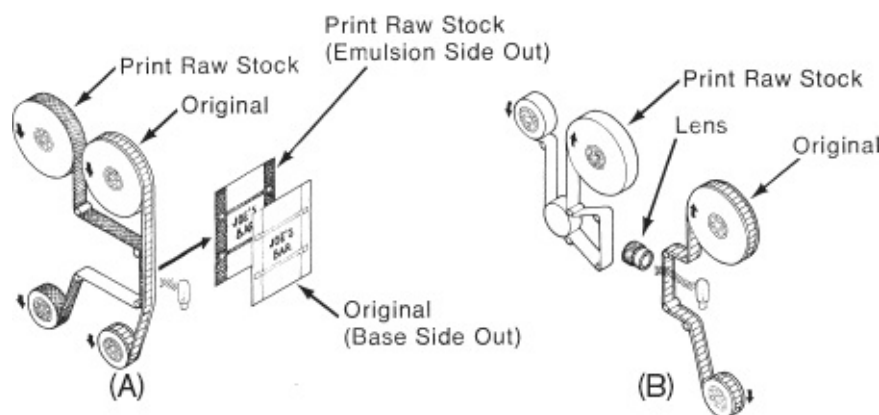
Fig. 16-12. Contact and optical printing. (A) The contact printer: the original is printed in emulsion-to-emulsion contact with the print stock. The inset shows how this changes the wind. Usually the original reads through the base (B-wind), and the contact print reads through the emulsion (A-wind). (B) The optical printer: a lens is used between the original and print stock. The wind can be preserved or changed on an optical printer. (Carol Keller)
