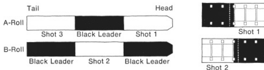
Fig. 16-13. A&B rolling. (left) Three shots laid out on A&B rolls with black leader as spacing. (right) The overlap for the 16mm cement splice occurs over the black leader, not over the picture. (Carol Keller)
