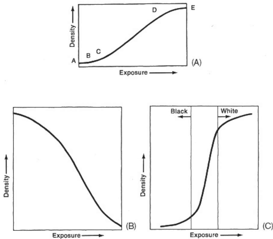
Fig. 7-3. Characteristic curves. (A) A simplified characteristic curve for black-and-white negative film: point A is the base-plus-fog density; B to C is the toe; C to D is the straight line portion; D to E is the shoulder. (B) Characteristic curve for reversal film. The greater steepness of the curve shows the higher contrast of reversal stock. (C) A very high-contrast black-and-white negative stock used for titles. (Carol Keller)
