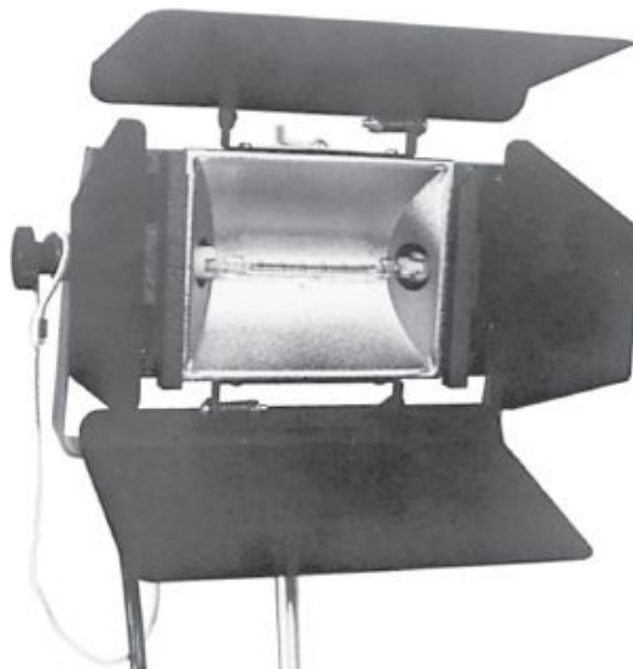
Fig. 12-18. Broad. Bardwell & McAlister 1,000-watt Mini-Mac with four-leaf barndoor. Note the tubular bulb. (Bardwell & McAlister, Inc.)
