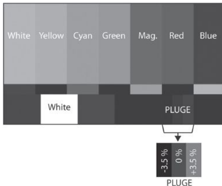
Fig. B. SMPTE HD split-field bars. The PLUGE is shown here with elevated blacks for clarity. Only the +3.5 percent stripe should be visible.
