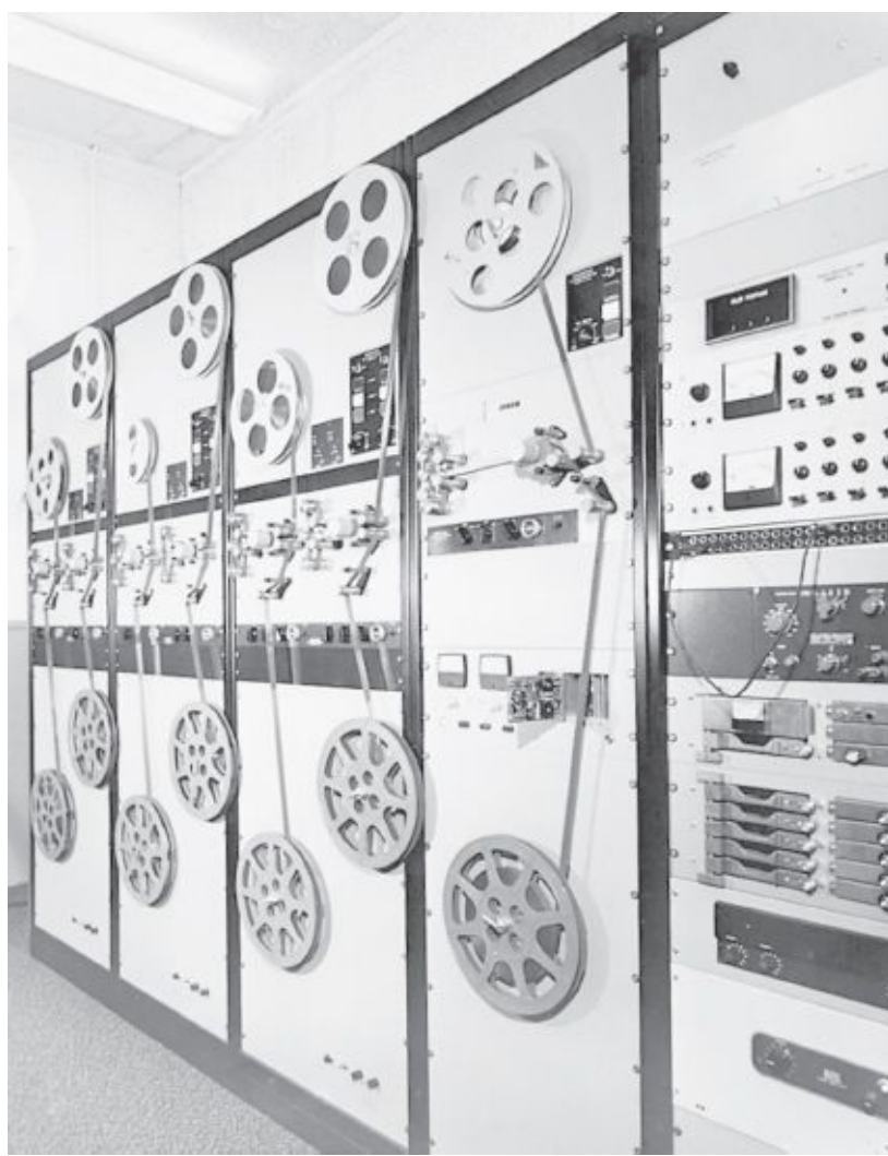
Fig. 15-11. For decades, film mixes were done with multiple reels of analog magnetic film playing on dubbers. Six playback transports are at left; one master record dubber is at right. Now, most of the dubbers that survive are only used to transfer mag film to digital for mixing. (Rangertone Research)
