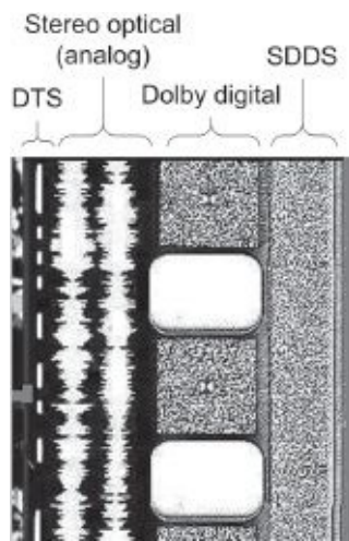
Fig. 16-16. The edge of a 35mm release print showing four types of analog and digital sound tracks that can be put on the same print. (Frank Angel)
