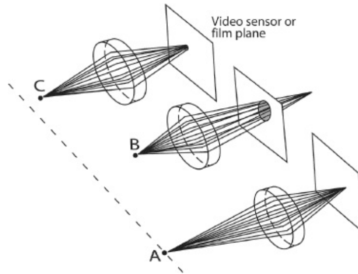
Fig. 4-10. Depth of field. All three lenses are focused at the dashed line. (bottom) Point A is on the line and the rays of light converge to a point at the video sensor. This is in sharp focus. (middle) Point B is closer to the lens so the rays of light form a circle ( circle of confusion ) where they hit the sensor. This is out of focus. (top) The rays of light from point C also form a circle, but it's small enough to appear as a point to the eye. This seems in focus to the viewer and thus C is within the depth of field. The same principle applies for a film camera; substitute the film for the sensor in the description above. (Steven Ascher)
