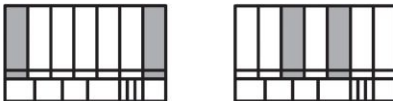
Fig. D. (left) With SMPTE HD split-field bars, when adjusting chroma on a monitor that displays blue only, these two bars and the patches under them should have the same intensity. (right) When adjusting hue (tint) for an analog signal, these bars and the patches under them should look the same. In the case of either a digital or analog input signal, when you finish setting up the monitor, these four bars and
