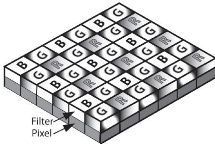
Fig. 1-13. In single-chip cameras, tiny colored filters are positioned over individual photosites (pixels) so that each one records either red, green, or blue light. In the commonly used Bayer pattern shown here, there are twice as many green pixels as either red or blue. The pixels are a bit like tiles in a mosaic, and prior to viewing the image, the data from the sensor must be “demosaicked” (also called “debayered”) to calculate full RGB color values for each pixel. For more on this, see p. 203 . (Steven Ascher)
