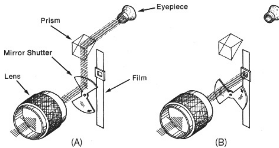
Fig. 6-7. Mirror shutter. (A) With the shutter closed, all the light is diverted to the viewfinder. (B) With the shutter open, all the light strikes the film and exposes it. Compare with Fig. 6-8. (Carol Keller)
