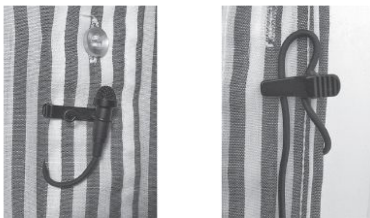
Fig. 10-25. When clipping a lav on clothing, make a loop with the cable under the clip in back to keep the cable neatly tucked in and to provide strain relief so any tugs on the cable won't pull directly on the mic.
