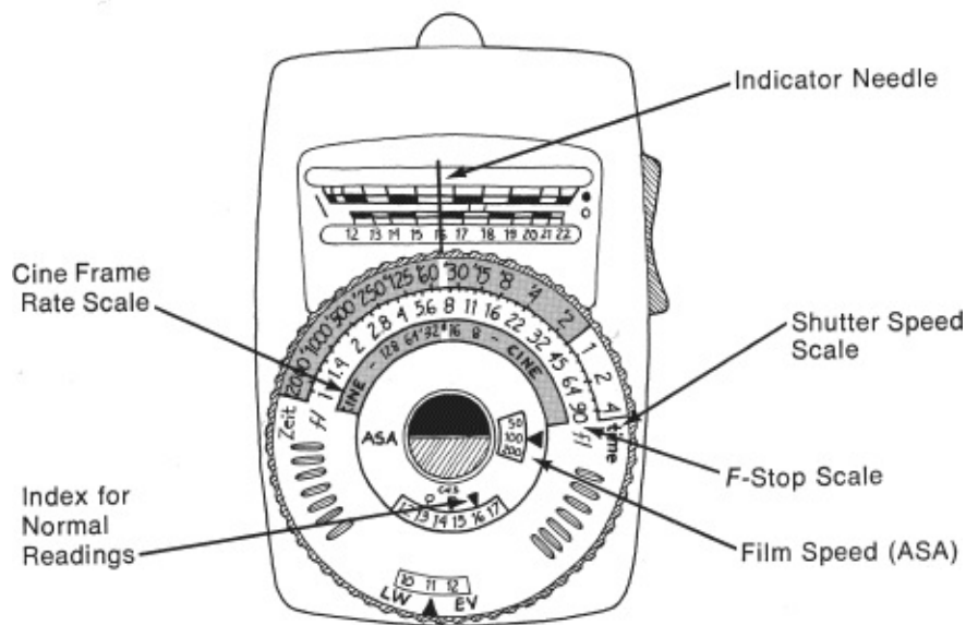
Fig. 7-13. Calculator dial found on Gossen Luna-Pro meter. The film speed window indicates that the meter is set for ASA 100 film. The light reading (16) is set opposite the triangle in the window just below the ASA setting. A camera with a 180-degree shutter run at 24 fps has a shutter speed of \frac{1}{50} second (50 can be found on the time scale between '60 and '30). The f -stop is read opposite this point. Alternatively, the f -stop could be read opposite the 24 fps mark on the cine scale (found between 32 and 16). The meter indicates a reading between f/5.6 and f/8 . (Carol Keller)
