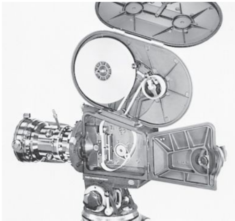
Fig. 6-1. Arriflex 16mm BL. The film chamber door and magazine lid are open to reveal the film path. The feed roll is 400 feet of core-loaded film. The pressure plate is open to show the film gate. The camera has a mirror shutter for reflex viewing. (ARRI, Inc.)
