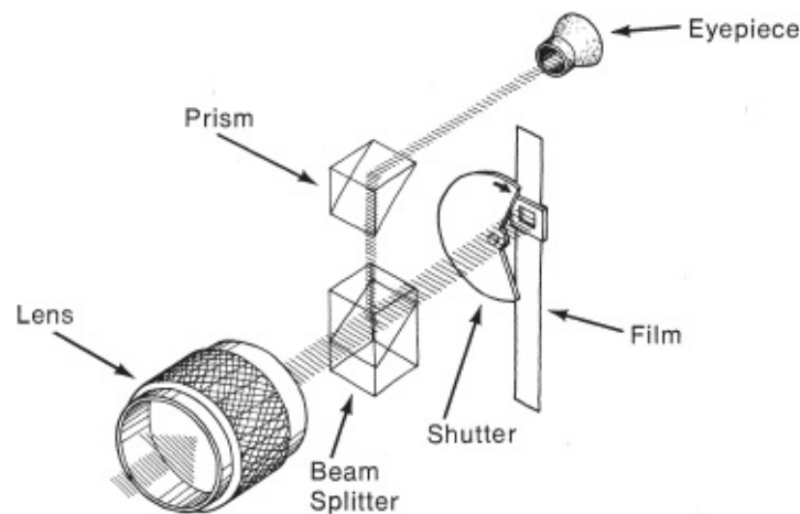
Fig. 6-8. Beam-splitter reflex. Some light is always diverted to the viewfinder, making it unavailable for exposing the film. (Carol Keller)
