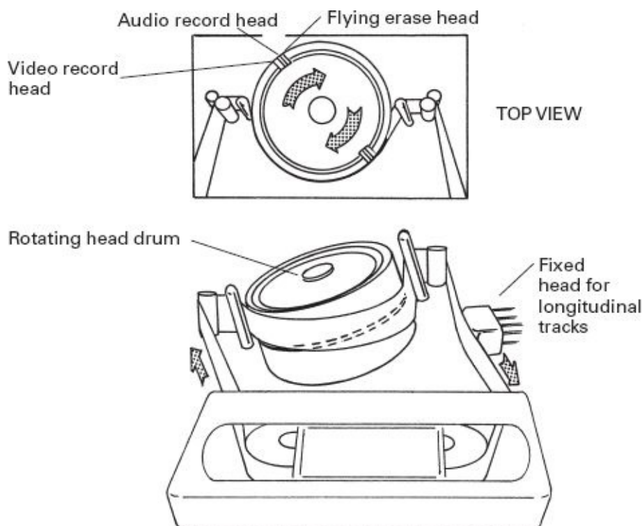
Fig. 3-10. Simplified view of the tape path and heads. Video formats vary widely in the configuration of the heads and the tape path. (Robert Brun)
