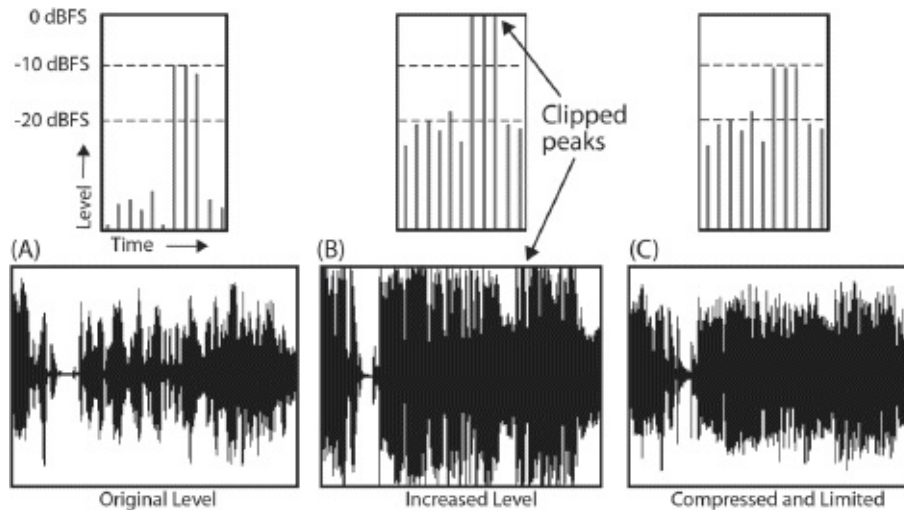
Fig. 15-14. Compression and limiting. (A) This audio has great dynamic range—note the difference in level between the quietest sounds and the peaks. (B) If we raise the level so that the quieter sounds are loud enough to be heard clearly, the peaks are now too high and will be clipped and distorted. (C) Using a compressor, we can reduce the height of the peaks while keeping the average level up. In this case, a limiter is also being used to ensure that no peaks go over -10 dBFS. Note that we've now significantly reduced the sound's dynamic range. Because the average level has been raised, C will sound a lot louder than A, even though the highest peaks are the same in both. (Steven Ascher)
