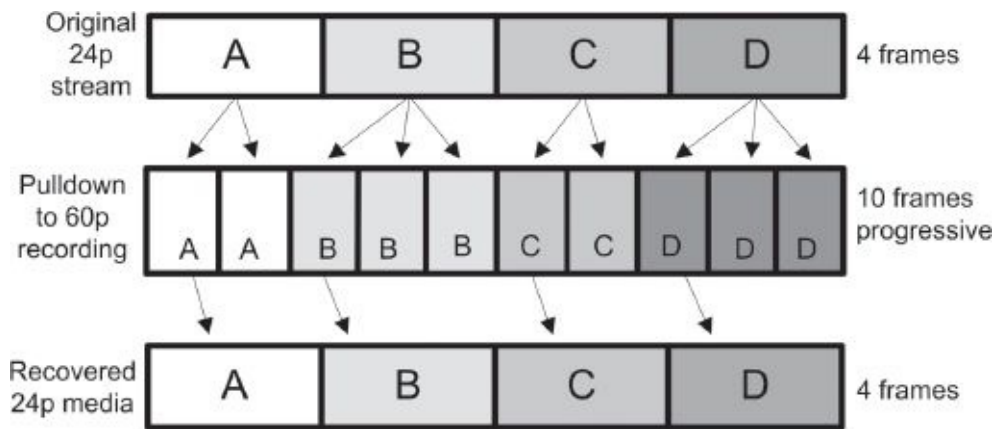
Fig. 14-33. 24p over 60p. The 720p HD format is always recording at 60 fps. When you shoot at 24p (top row), pulldown is used to record each frame either twice or three times in the 60p recording (and each recorded frame is a complete, progressive frame—not divided into fields as shown in Figs. 14-30, 14-31, and 14-32). To re-create the 24p stream, the system simply ignores the extra recorded frames in the middle row.
