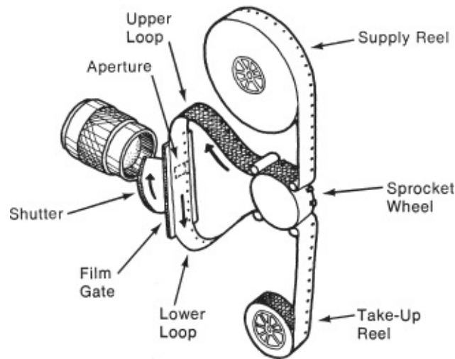
Fig. 6-2. Simplified camera. (Carol Keller)
