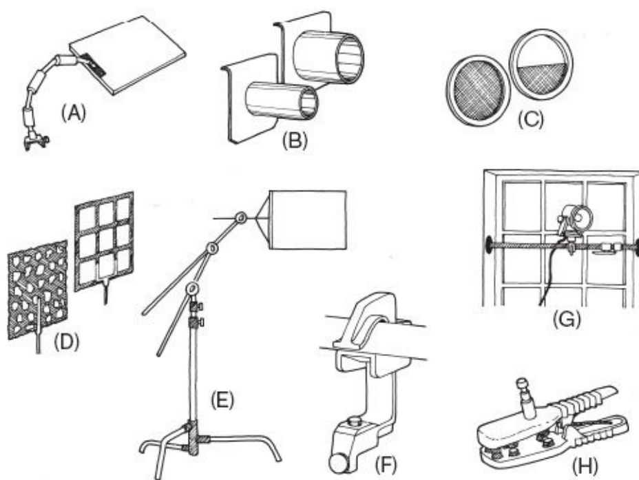
Fig. 12-24. Lighting accessories. (A) French flag. (B) Snoots. (C) Full scrim and half scrim. (D) Cookies. (E) Century stand with three gobo heads and flag. (F) Hanger for mounting on pipes or small beams. (G) Polecat mounted in window well. (H) Gator grip. (Representations are not drawn to same scale.) (Carol Keller)
