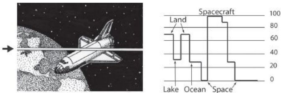
Fig. 5-4. By looking at the waveform display of a single horizontal line of pixels, you can more clearly see how luminance values in the image are represented in the waveform monitor. (Robert Brun)
