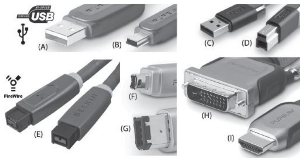
Fig. 5-29. Data and video connectors. (A) USB 2.0 male A connector. (B) USB 2.0 Mini B connector. (C) USB 3.0 male A connector (USB 3.0 is faster than 2.0 but this connector is backward compatible with 2.0 ports). (D) USB 3.0 male B connector. (E) FireWire 800 (IEEE 1394). (F) FireWire 400 four-pin connector. (G) FireWire 400 six-pin (the two extra pins supply power). (H) DVI connector. (I) HDMI connector. For other common connectors see Figs. 3-14 , 10-13 , and 10-32 . (Belkin Corporation)
