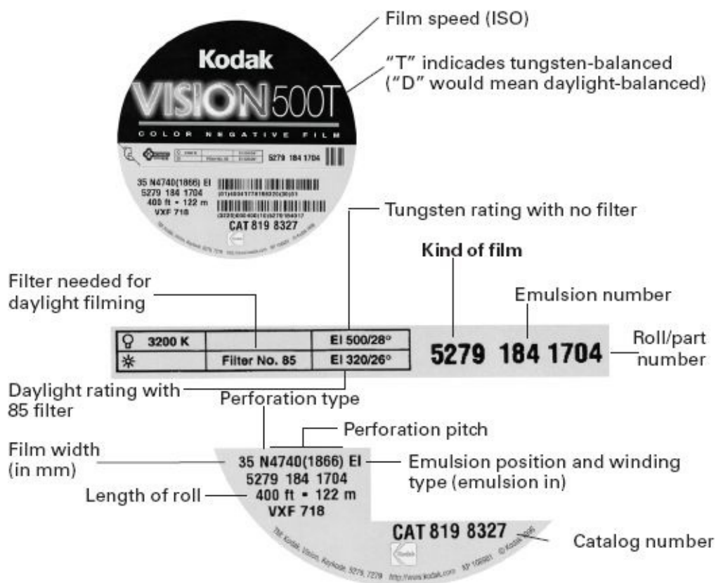
Fig. 7-7. Film label and enlarged details. This label is for Kodak 5279 color negative film, also called Vision 500T (now discontinued). The newer version is 5219 (Vision3 500T). (Eastman Kodak Company)
