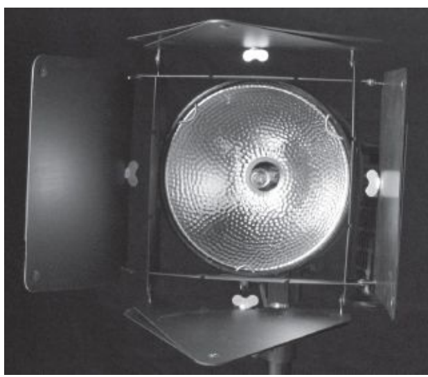
Fig. 12-17. Lowel DP open-faced spot. The quartz bulb is clearly visible. (Lowel Light Mfg., Inc.)
