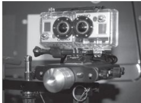
Fig. 9-53. Side-by-side 3D rig. This one uses two GoPro Hero HD cameras (see Fig. 2-8 ). (Photo by David Leitner)
