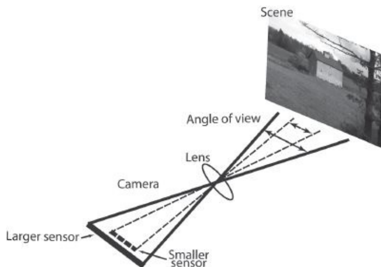
Fig. 4-6. Angle of view and sensor size. If two cameras have the same focal length lens, the camera with the smaller sensor will see the scene with a narrower angle of view than the camera with a larger sensor. With film cameras, the same principle applies to wider and narrower film formats. See the results in Fig. 4-7. (Steven Ascher)
