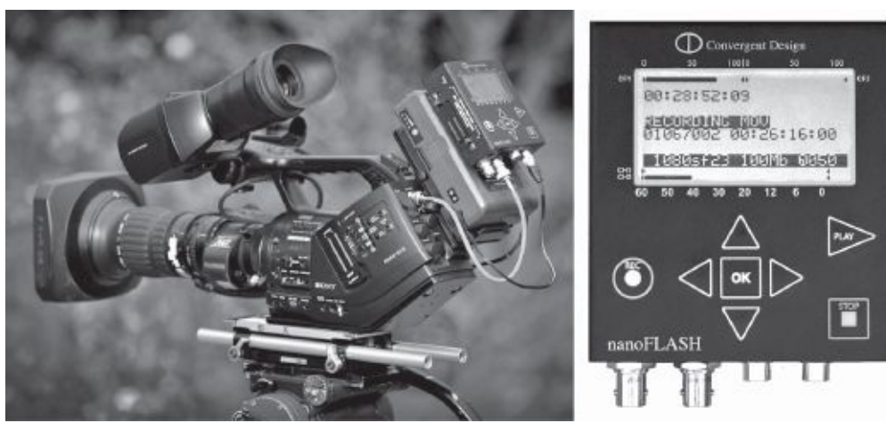
Fig. 1-27. Sony EX3 camcorder records XDCAM EX to internal memory cards, but can record less compressed formats when used with an external recorder such as the nanoFlash unit pictured here. In this shot, a high-capacity V-mount battery is mounted between the camera and the recorder. (George T. Griswold; Convergent Design)
