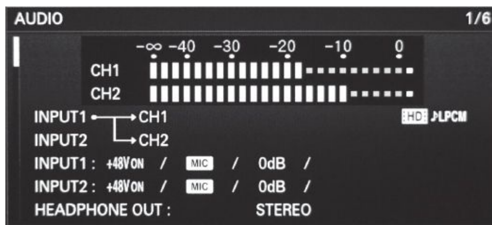
Fig. 11-7. Digital peak-reading meter. You never want the level to reach 0 dB. When the dot to the right of 0 lights up, the sound will be clipped. Indicators below the meter show that Input 1 is going to both recording channels, the mic is being fed +48 volt phantom power, and the camera is recording PCM uncompressed audio.
