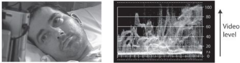
Fig. 5-3. A waveform monitor displays video levels in the image. In this case, you can see that the brightest parts of the bed sheet on the right side of the frame are exceeding 100 percent video level. (Steven Ascher)
