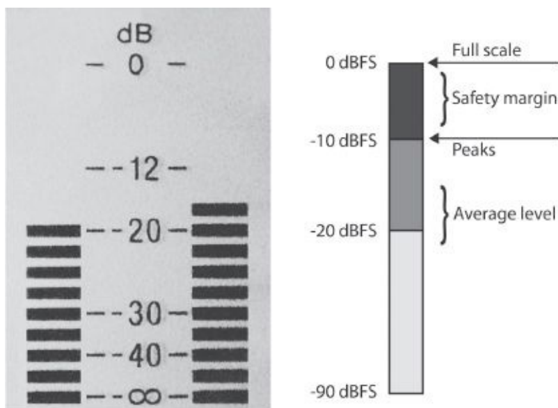
Fig. 11-10. (left) Peak-reading meter. The left channel reads -20 dBFS. (right) Rough guidelines for setting the level during field recording. Average level is around -20 dBFS or so with typical peaks reaching up to -10 dBFS. This leaves a safety margin of 10 dB for unexpectedly loud peaks. Different situations call for different levels.
