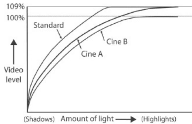
Fig. 5-9. Gamma curves. Standard gamma rises quickly in the shadows, creates relatively bright midtones, and reaches the white clip level relatively soon. By comparison, the Cine A curve provides darker shadows and midtones but continues to rise to the right of the point at which the standard curve has stopped responding, so it's able to capture brighter highlights. The Cine B curve is similar to Cine A, but tops out at 100 percent video level, so the picture is legal for broadcast without correction in post. These curves are for illustration only; the names and specific gamma curves in your camera may be different. (Steven Ascher)
