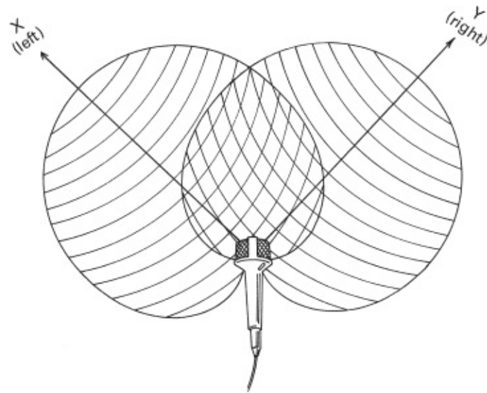
Fig. 11-14. Pickup pattern of a stereo mic in the X-Y configuration. Shown here, the two mic capsules are in one body. (Robert Brun)
