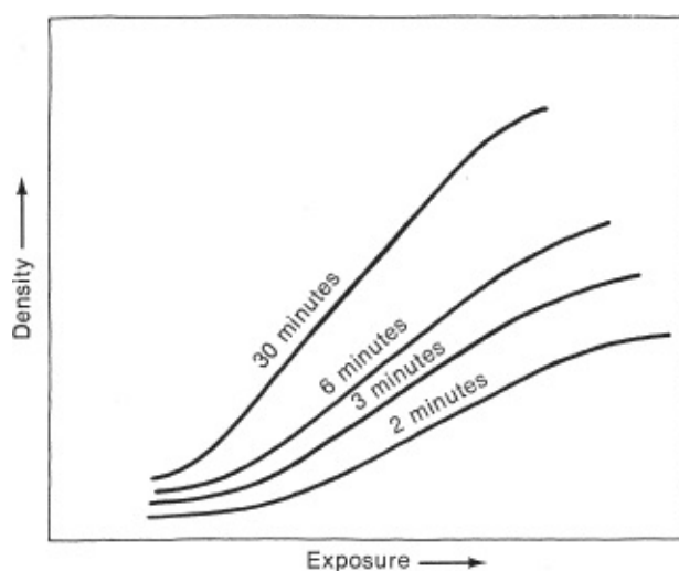
Fig. 7-6. Force processing. As the development time increases, the characteristic curve becomes steeper (contrast increases)—because the brighter parts of the scene (right side of graph) respond more to increased development than the darker parts. Fog level also increases with development time. (Carol Keller)
