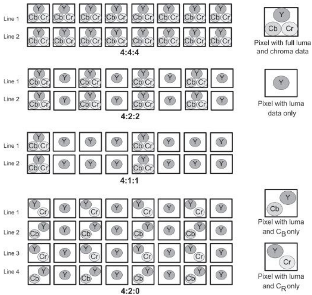
Fig. 5-15. Color sampling. In a 4:4:4 system, every pixel contains a full set of data about brightness (Y) and color (C B and C R ). In 4:2:2 and 4:1:1 systems, increasing amounts of color data are thrown away, resulting in more pixels that have only brightness (luma) information. In 4:2:0 systems, pixels with Y and C R alternate on adjacent lines with ones that have Y and C B (shown here is PAL DV; other 4:2:0 systems use slightly different layouts).
