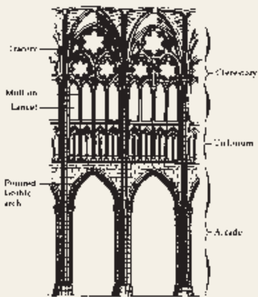
Gothic Church Interior Elevation
