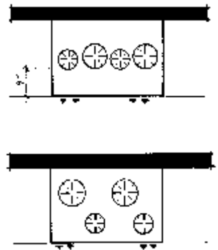
Figure 2.17 These two cooktop arrangements allow a wheelchair-bound person to use all elements without the danger of burns from reaching over the top of a heated element. Controls are on the front of the stove, assuring both ease of use and safety against burns.
