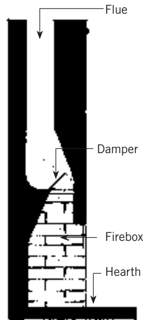
Figure 10.49 Fireplace components.
