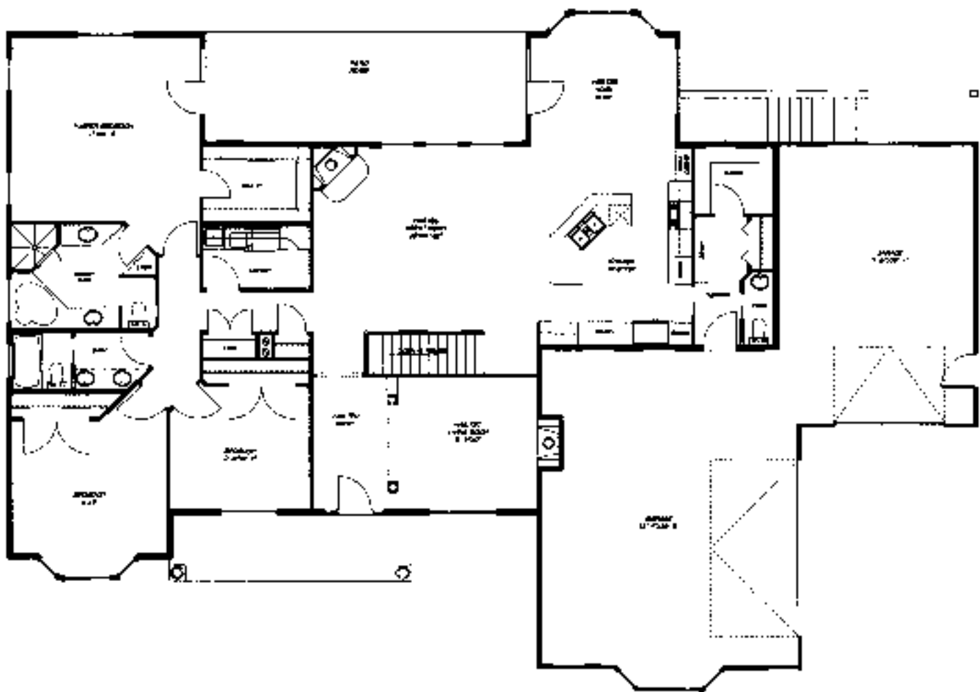
Figure 7.5 A ramblor or ranch-style plan with optional basement. CAD by Gary Stewart
