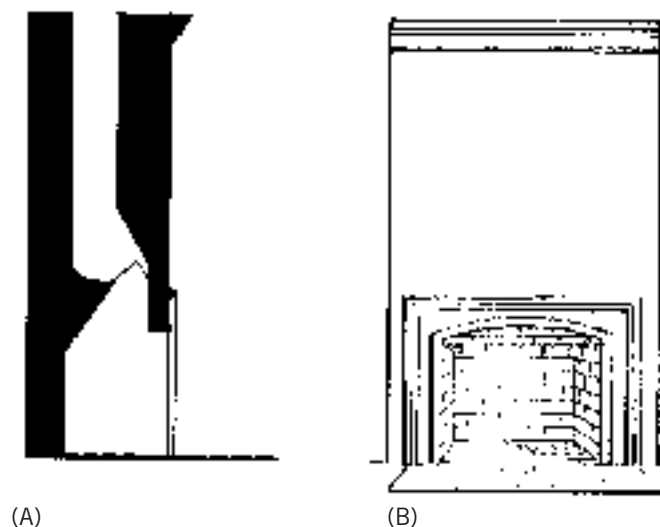
Figure 10.50 Flush-face fireplace. (A) Side cutaway section view. (B) Front view elevation.
