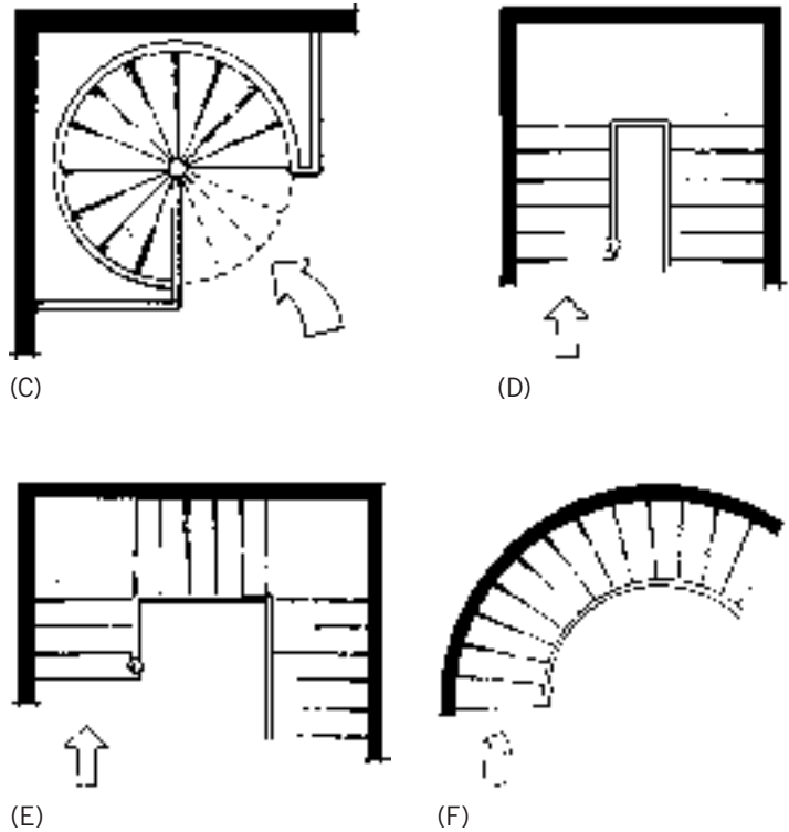
Figure 10.47 Stair forms. (A) Straight-run stair. (B) One-turn stair (with landing). (C) Spiral staircase. (D) U-stair (with one landing). (E) Double-turn stair (with two landings). (F) Semi-housed curved stair.
